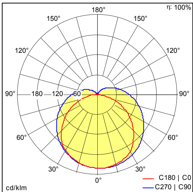
TE_POPPY_LED_1800_8500_840_E3e.ltd
