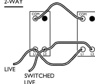
EXAMPLE WIRING 2-WAY
