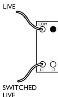
EXAMPLE WIRING 1-WAY
