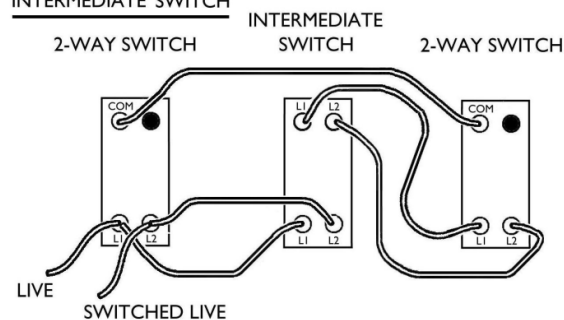
EXAMPLE WIRING INTERMEDIATE SWITCH
