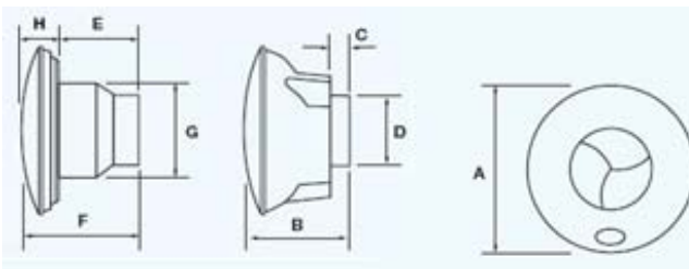
Recessed mounted Surface mounted
