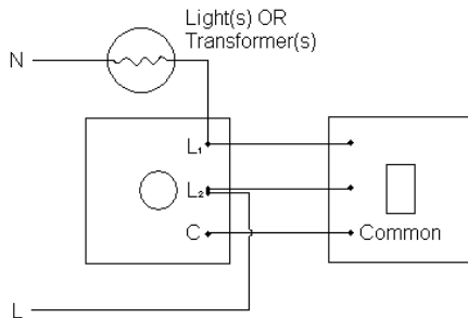
Figure 2. Using a 2-way Dimmerswitch. Dimmer must replace only one of the 2-way switches.
