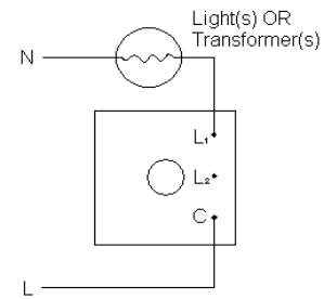
Typical 1-way Circuits (For single dimmerswitches or each module of a multi-gang dimmerswitch)
