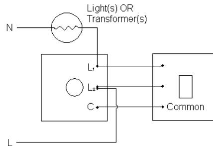
Figure 3. Using a 2-way Dimmerswitch. Dimmer must replace only one of the 2-way switches
